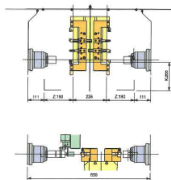
Stroke Diagram (Linear Turret)
